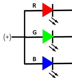
Common Anode (+)
