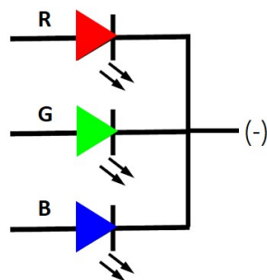
Common Cathode (-)
